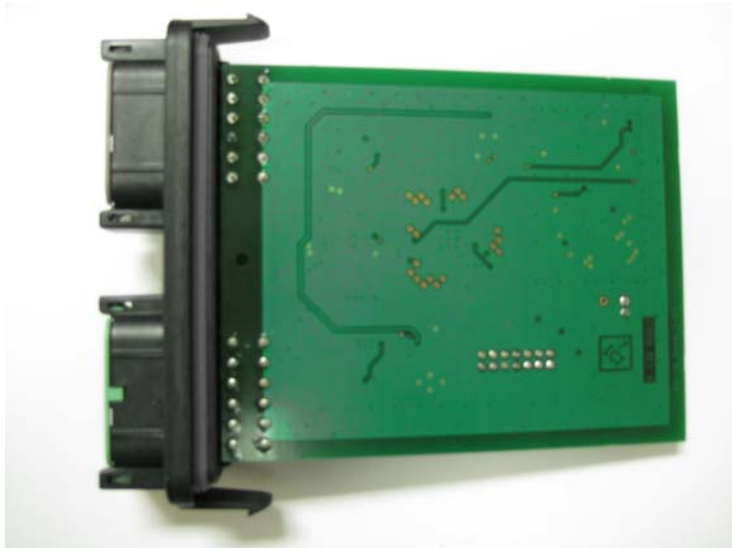
View #2 – Backside of RF Section
