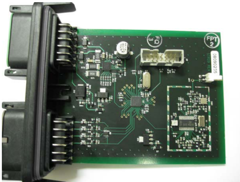
View #1 – RF Section, Shield Removed
