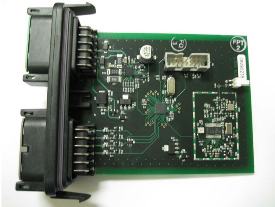
View #2 – RF Section, Shield Removed
