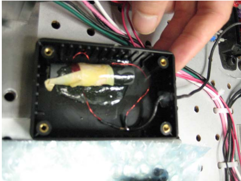
Wire Antenna
