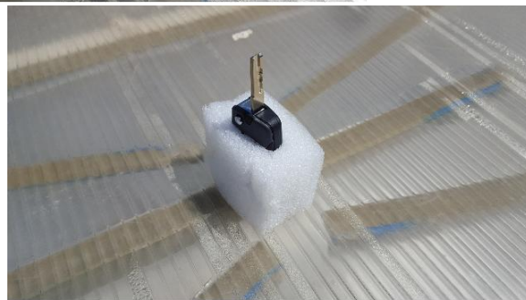
Figure 4: Radiated Emissions Test Setup Photograph(s).
