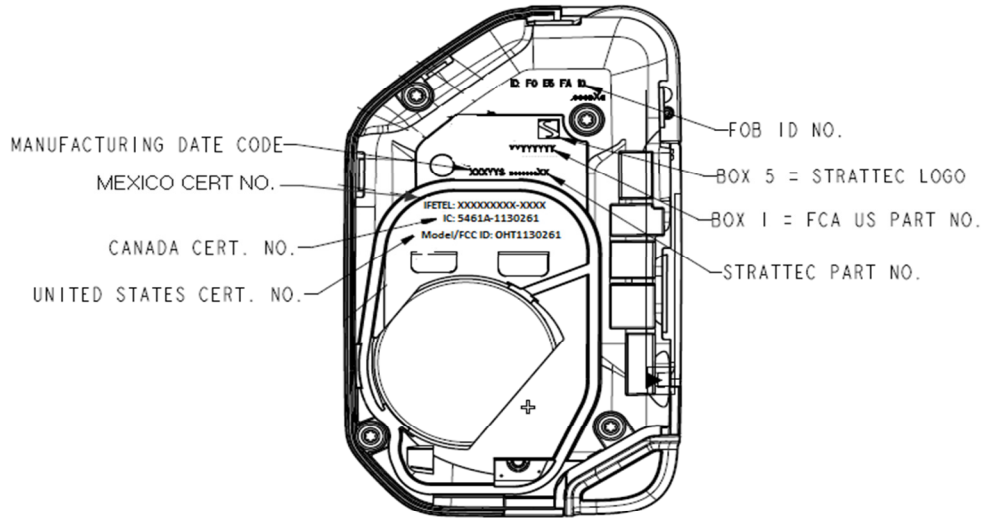
VARIANT: 433MHz MULTIPLE COMPONENTS REMOVED FOR CLARITY
