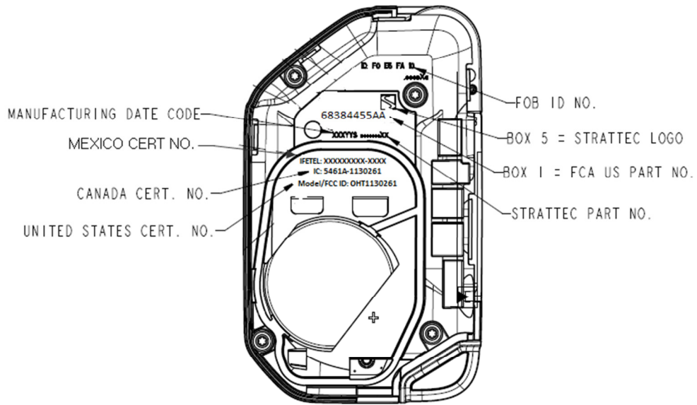
VARIANT: 433MHz MULTIPLE COMPONENTS REMOVED FOR CLARITY
