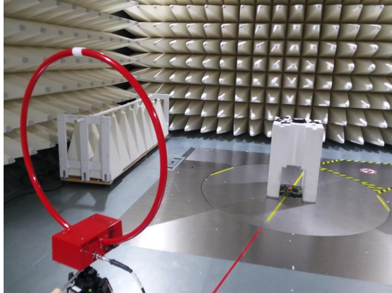
Figure B4: Radiated setup using Loop Antenna
