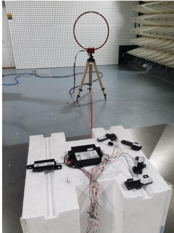
Figure B3: DUT Setup inside chamber
