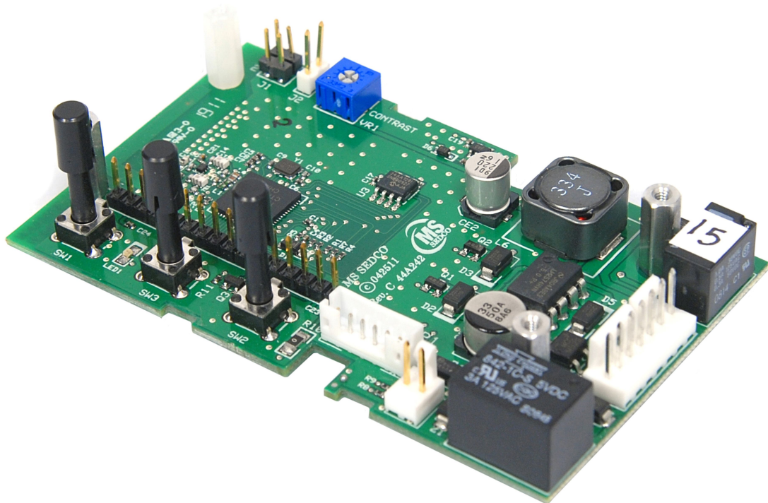
COORDINATOR PCB TOP
