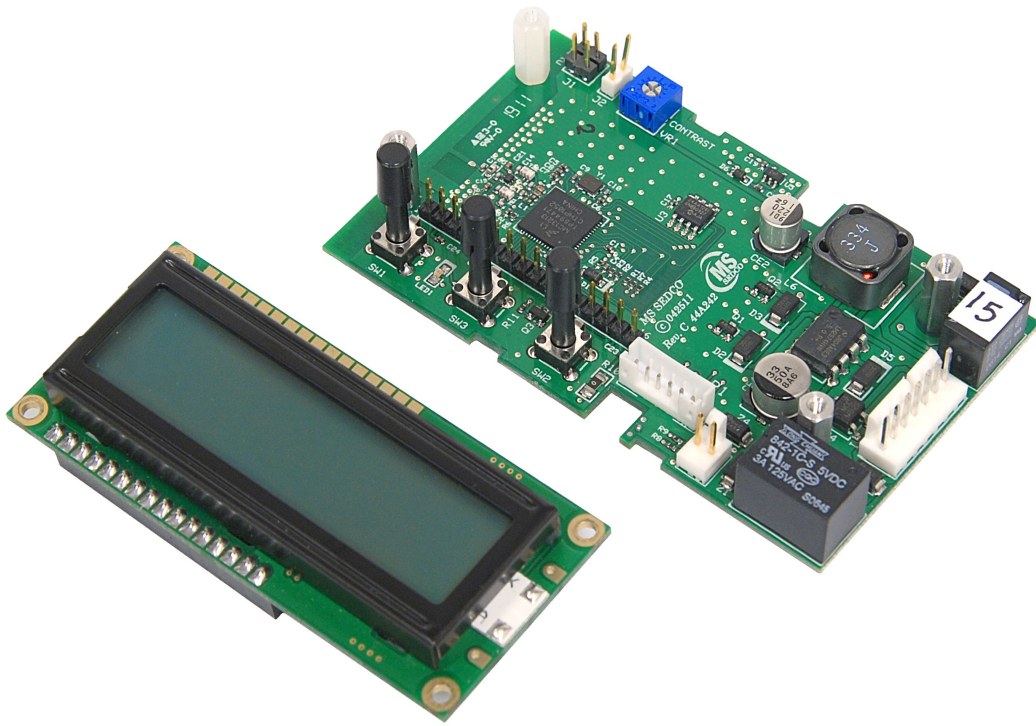
COORDINATOR AND DISPLAY PCB TOP
