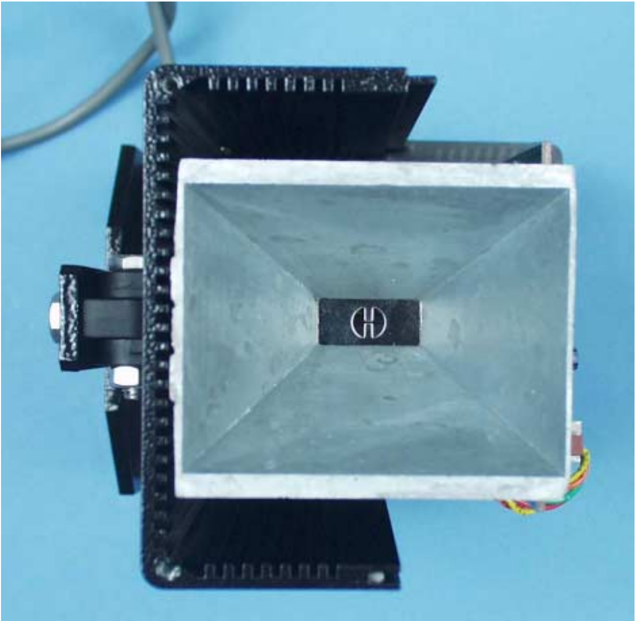
Internal Horn
