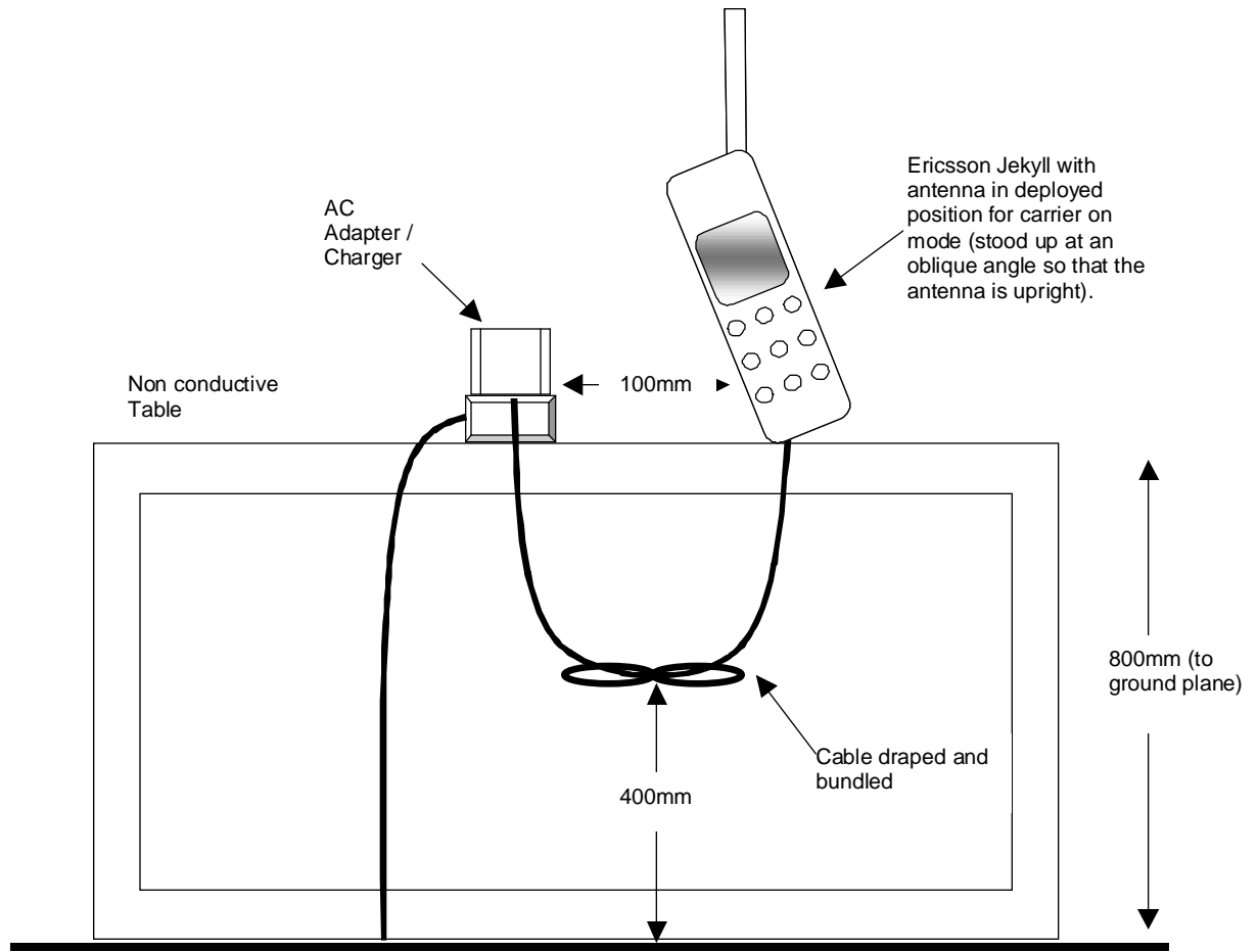
Figure 4: Ericsson Jekyll CFR 47 Part 25 Radiated Emission Set up (Rear View)
