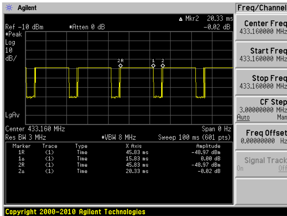
Duty Cycle
