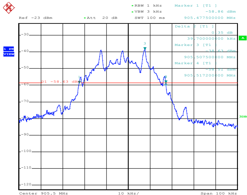
20 dB bandwidth
