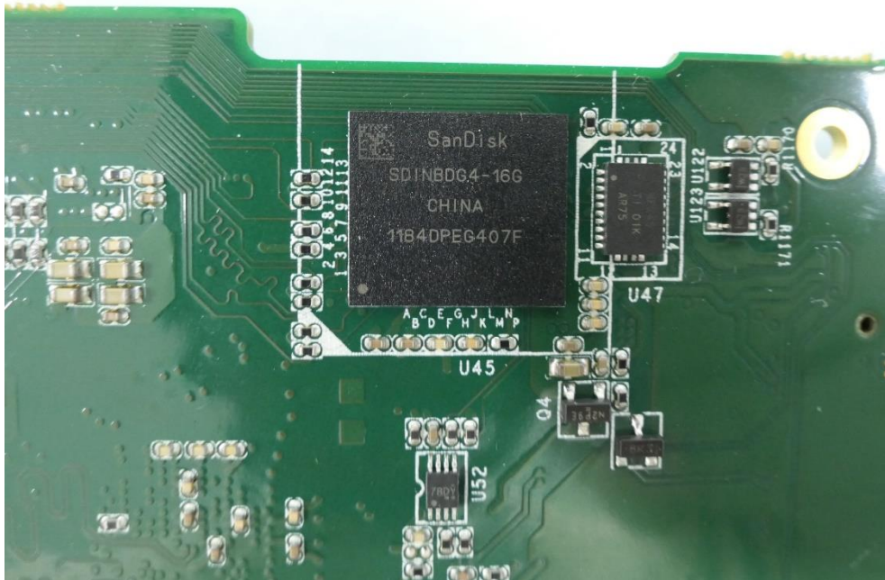
(32) EUT Photo
