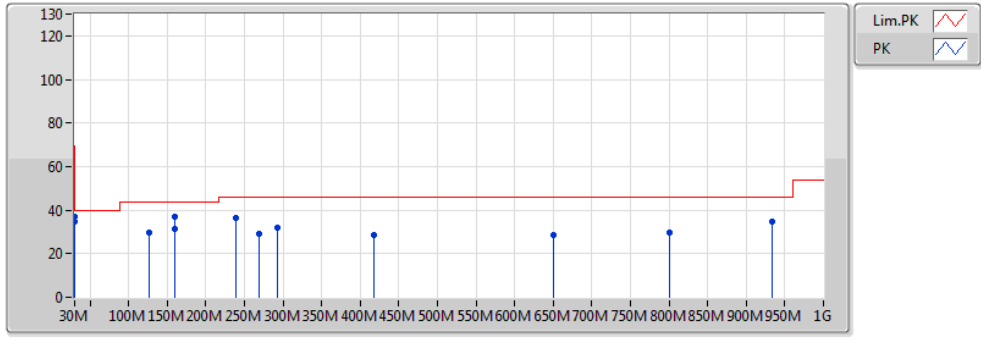
RE TX below 1GHz;Band:2.4G;BT-LE;BWch:1MHz;Nss:1;Nant:1;Ch:2440MHz; AC Adapter
