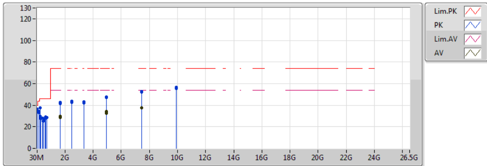
RE Co-TX or Cabinet;Band:2.4G;BT-LE;BWch:1MHz;Nss:1;Nant:1;Ch:2480MHz;TX 836.4MHz WCDMA BAND5
