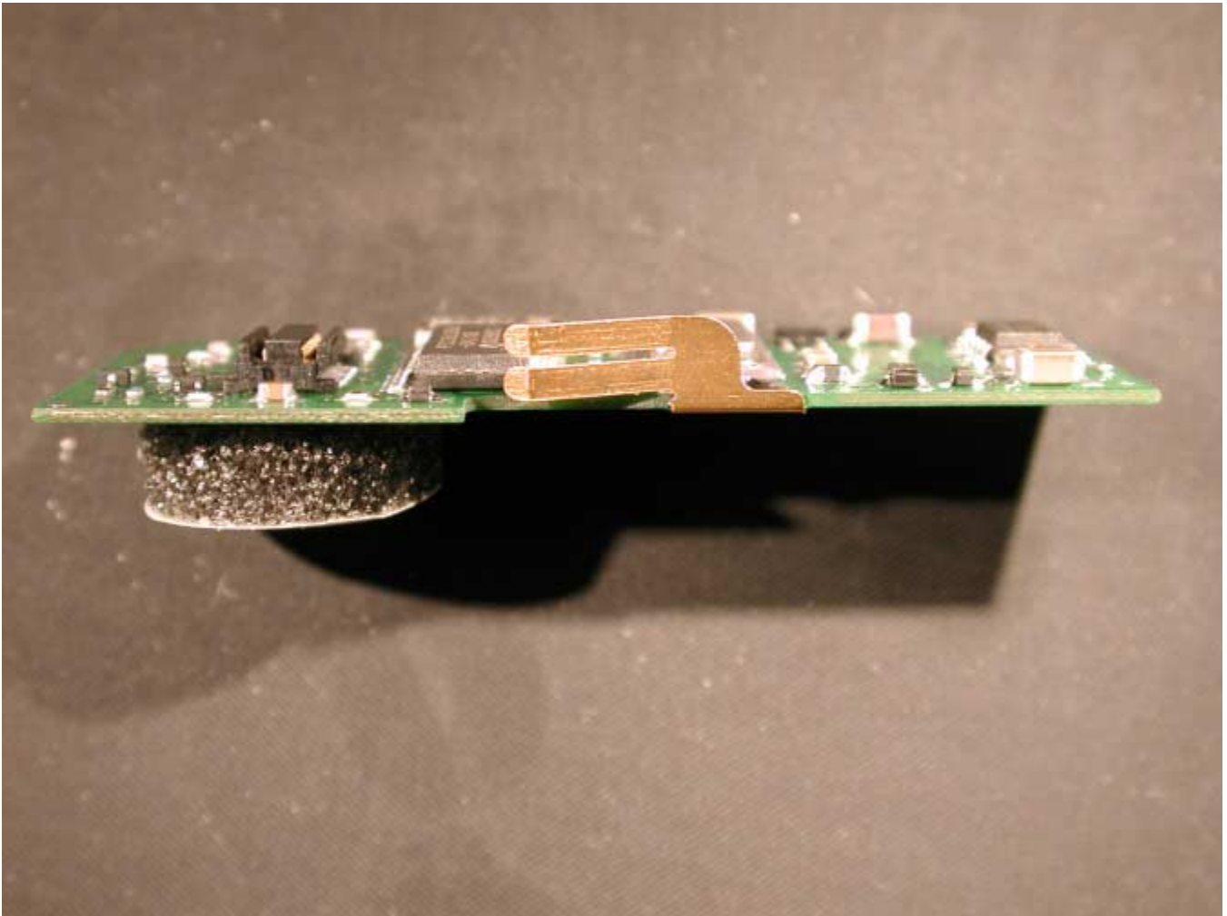
RF ANTENNA
