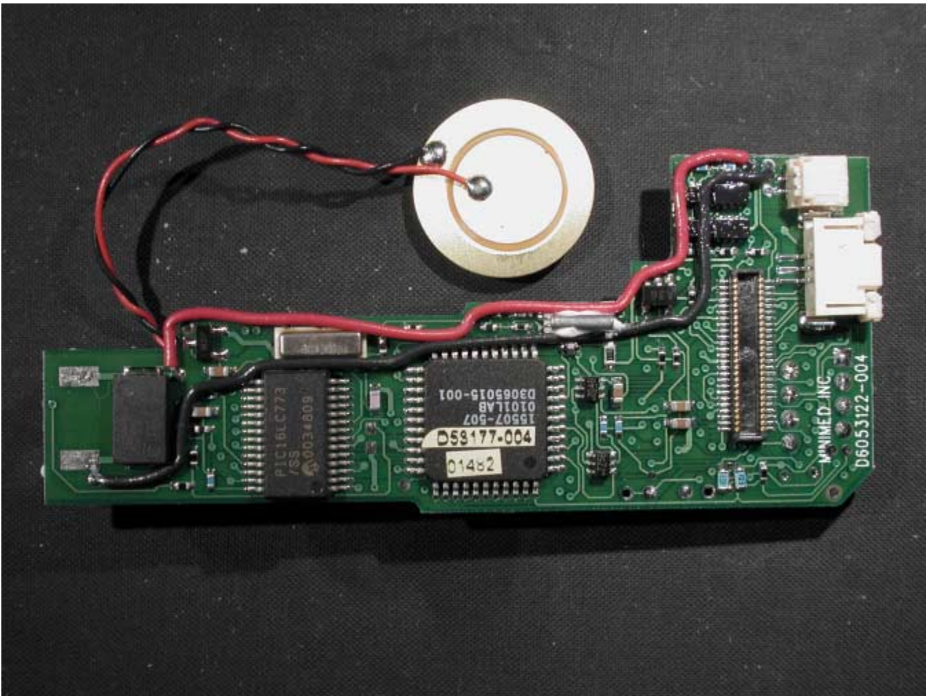
INTERFACE FRONT
