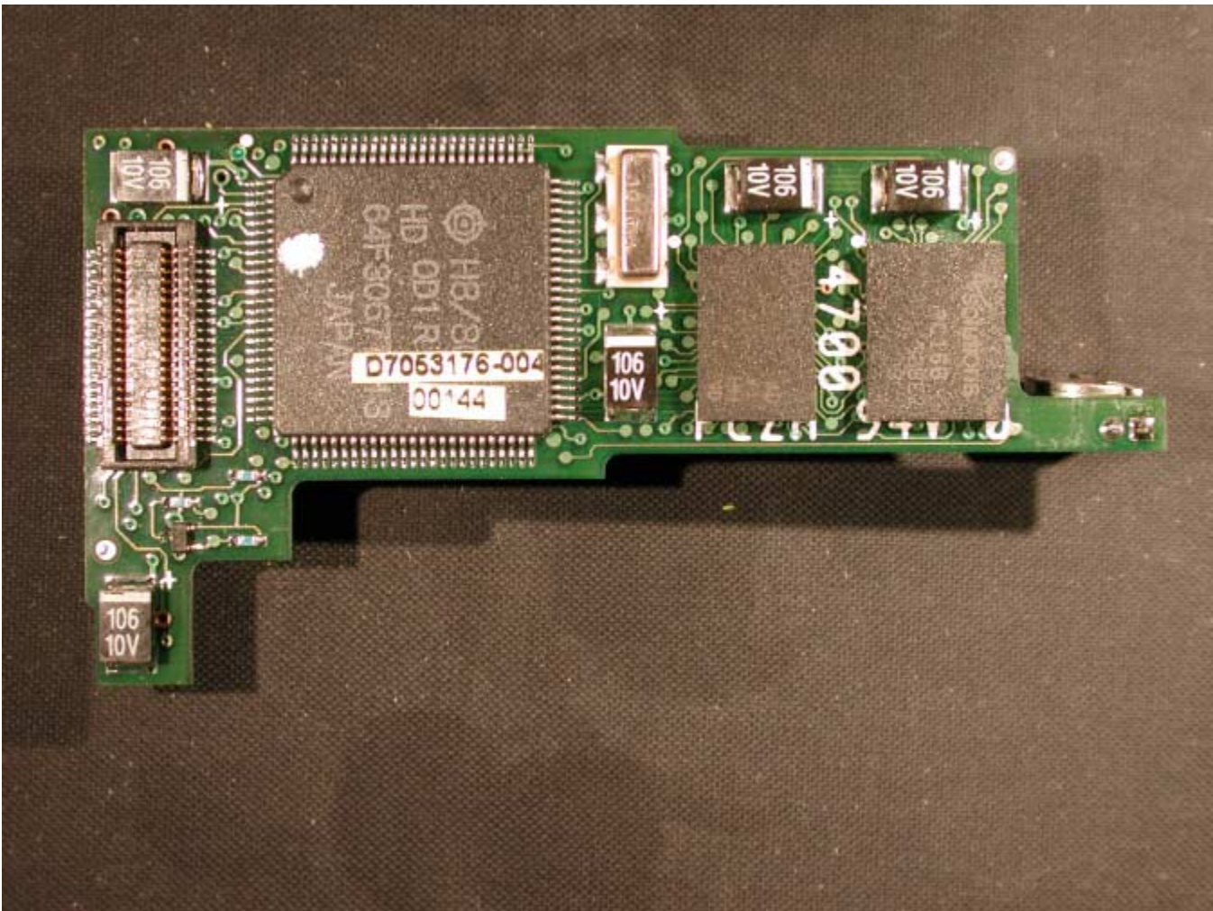
MOTHER FRONT
