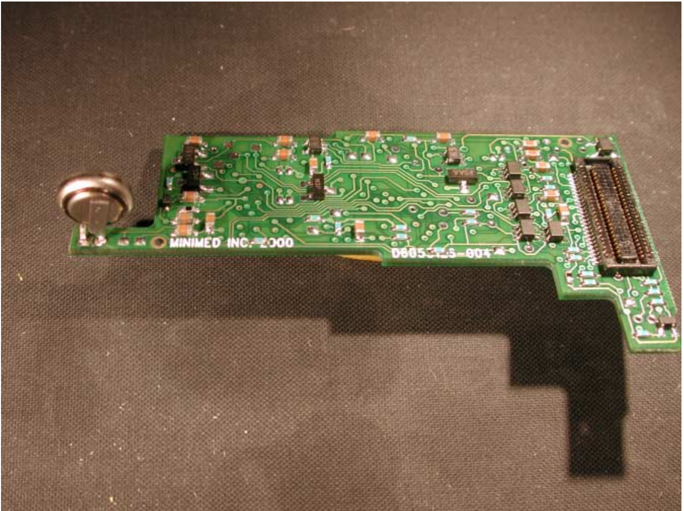
MOTHER OBLIQUE
