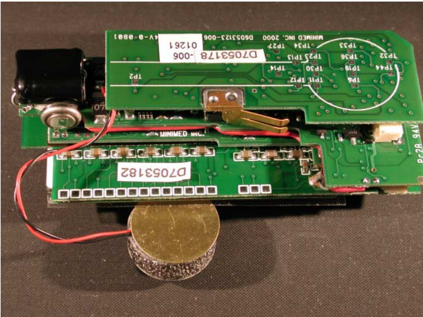
BOARDS STACKED 3
