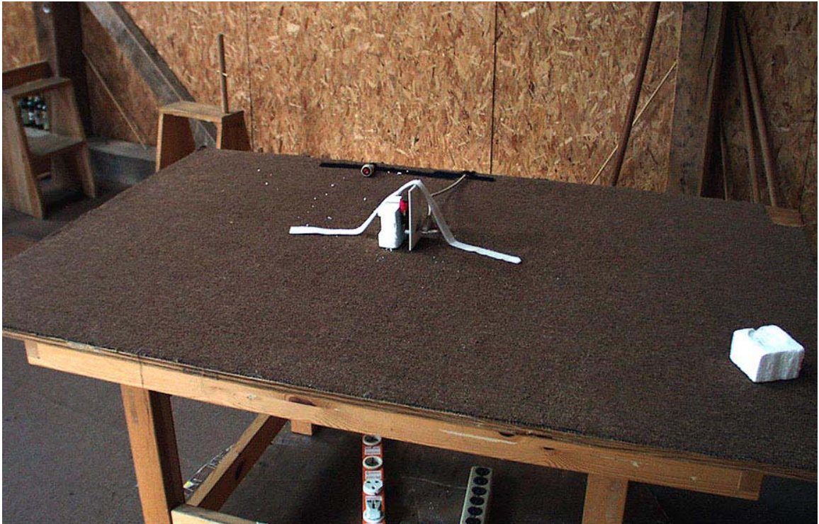
RADIATED SETUP END POSITION
