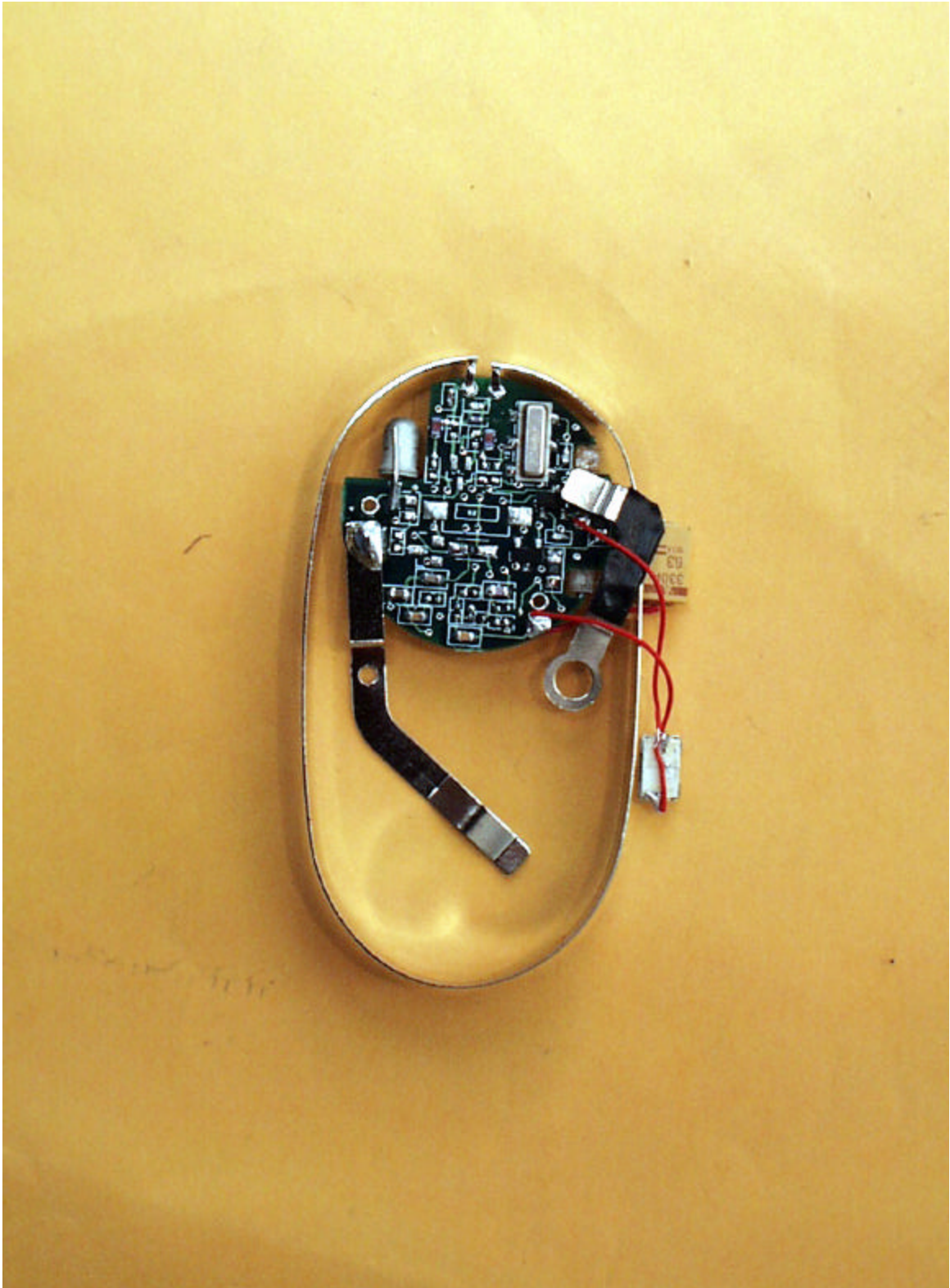
VER-1780 PCB – BOTTOM VIEW
