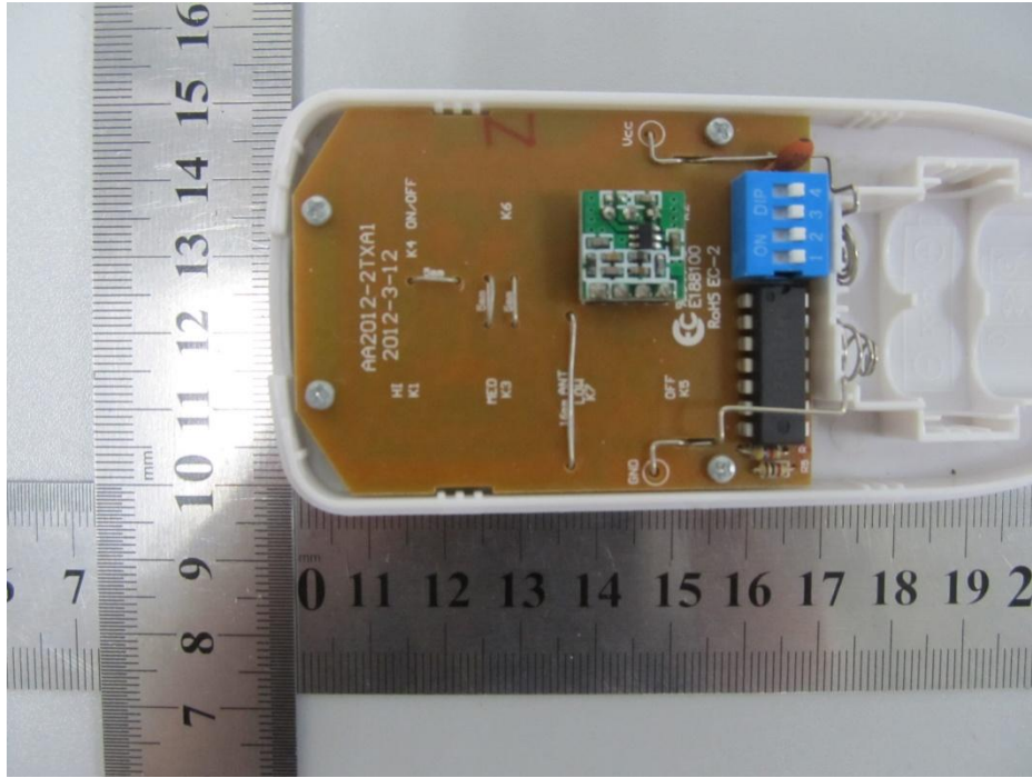
Internal Photo of AA1T3/AA2T3/AA3T3
