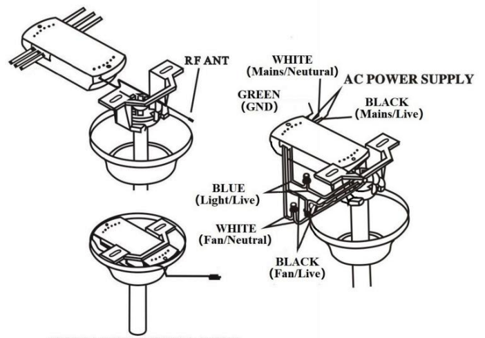
VIEW AFTER INSTALLATION
