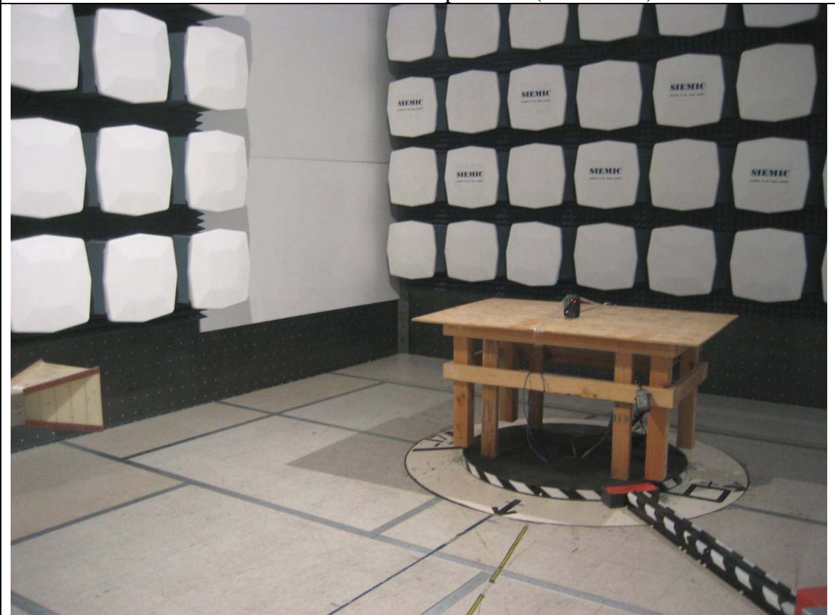
Radiated Emission Test Setup – View (>1000MHz)
