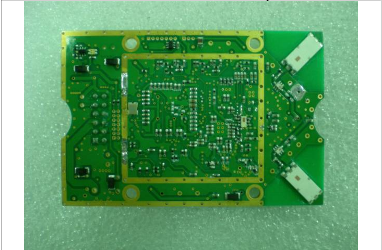
Radio Board Top View (Without Shielding)
