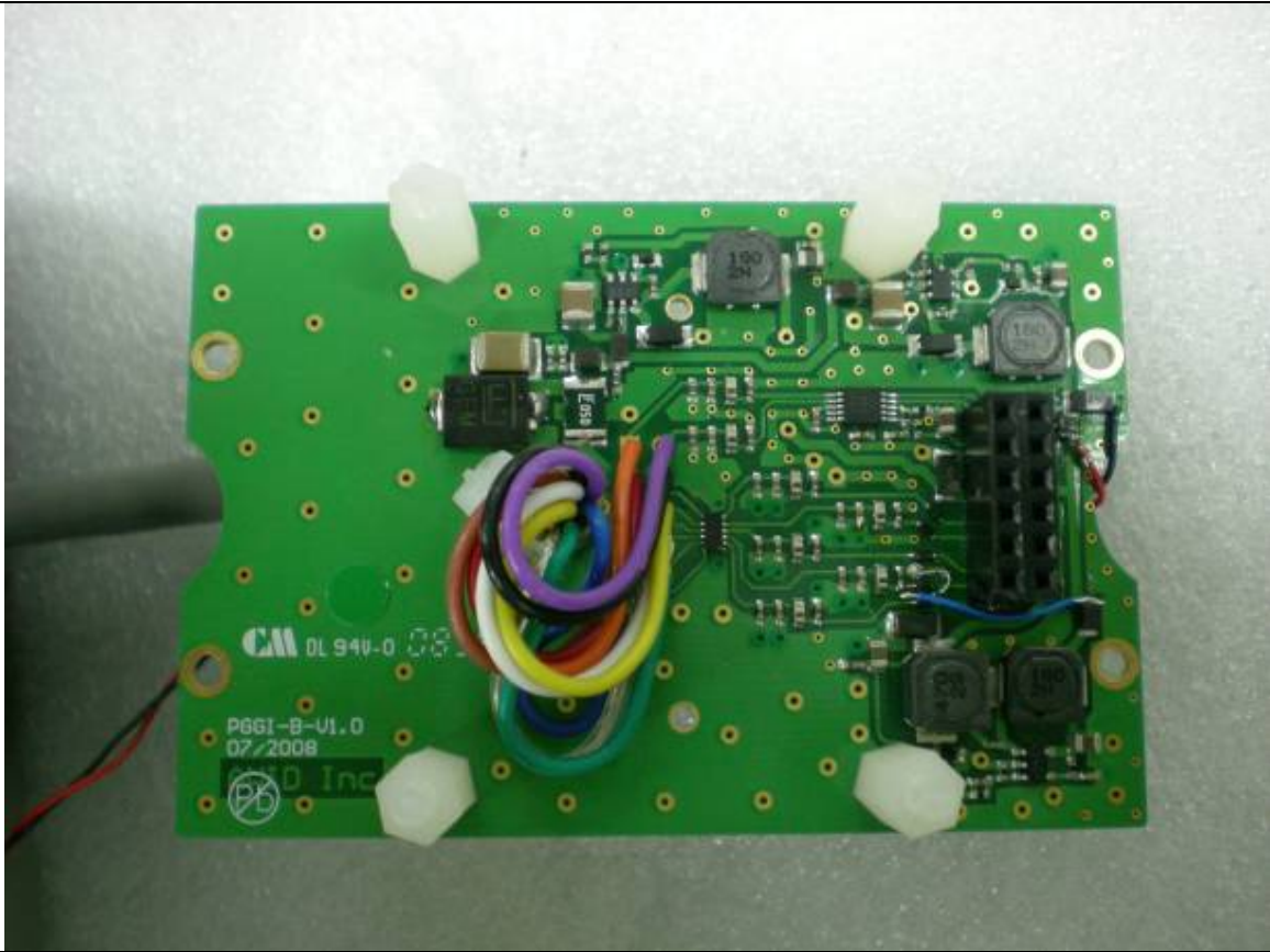
Control Board Bottom View
