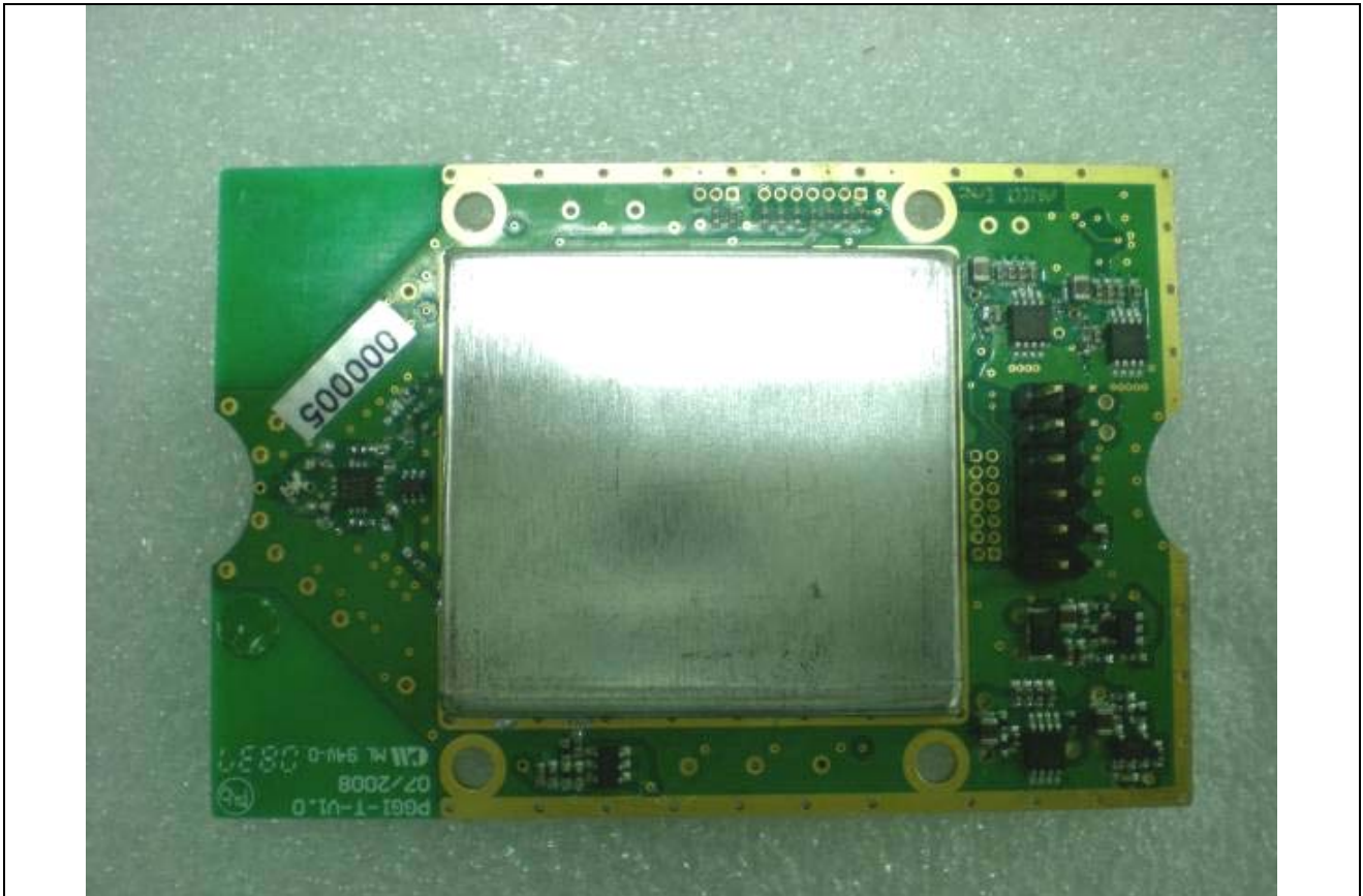
Radio Board Bottom View (With Shielding)
