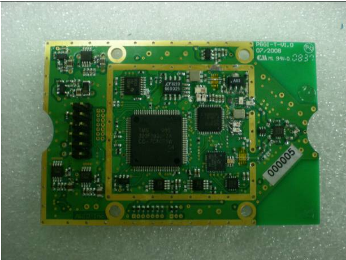
Radio Board Bottom View (Without Shielding)
