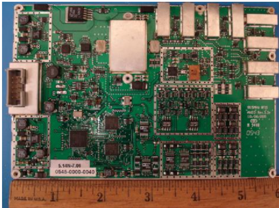
RF MAIN BOARD – TOP SIDE with SHIELD
