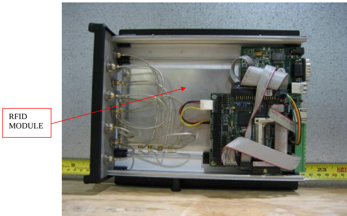
MODULE INSIDE OF CHASSIS
