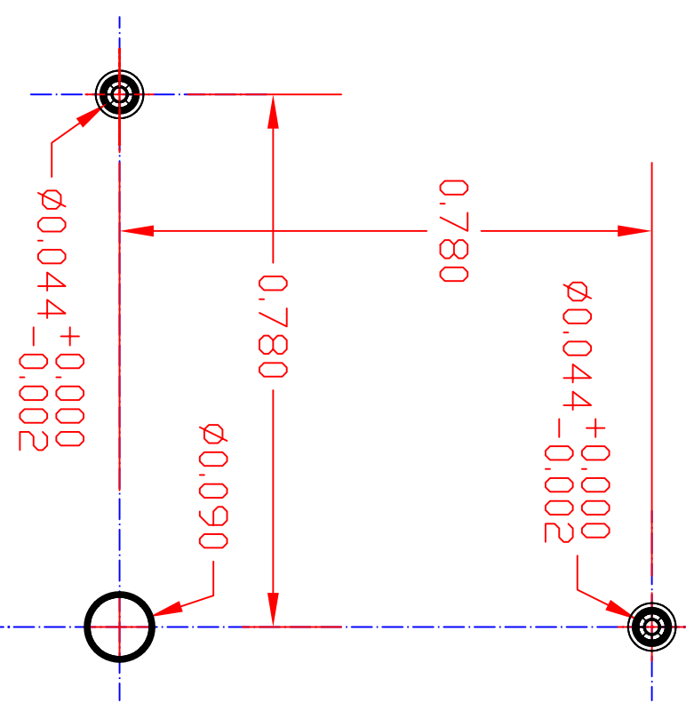
View A
