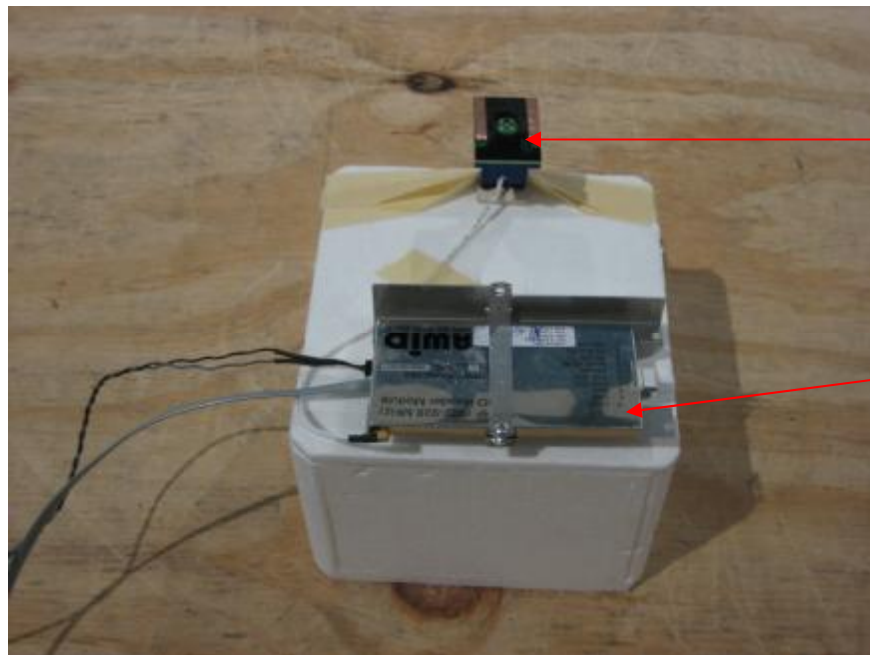
Radiated Emission setup (close-up)
