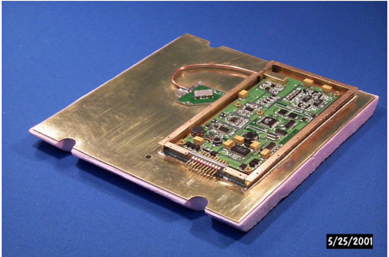
LR-911 without Shield and Cover
