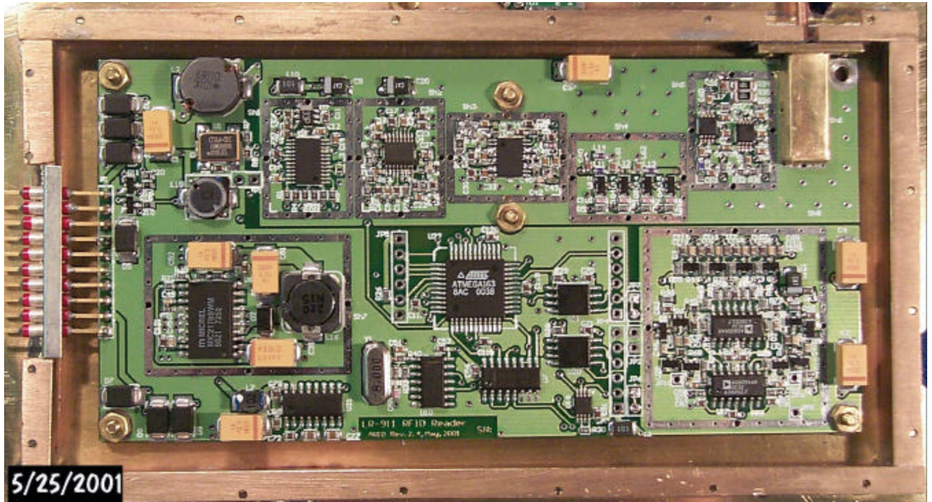
LR-911 PC Board Top View
