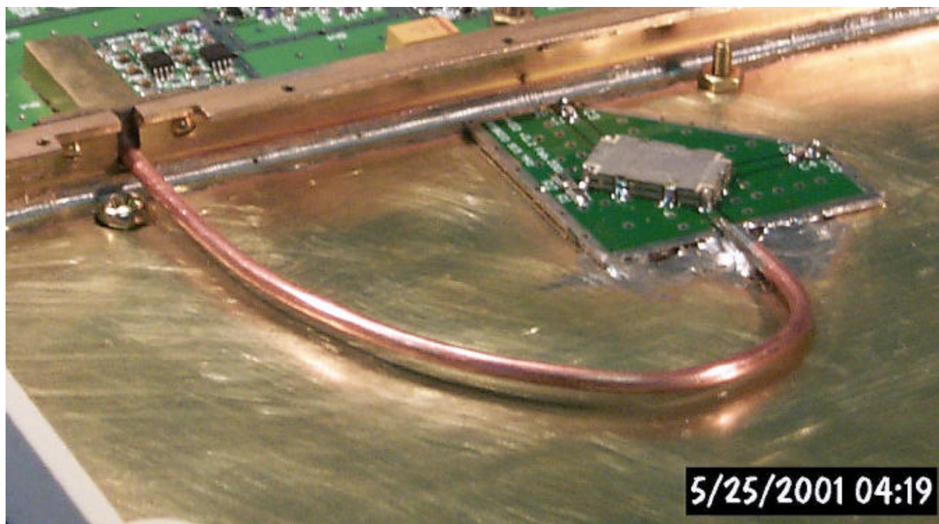
Antenna Connection
