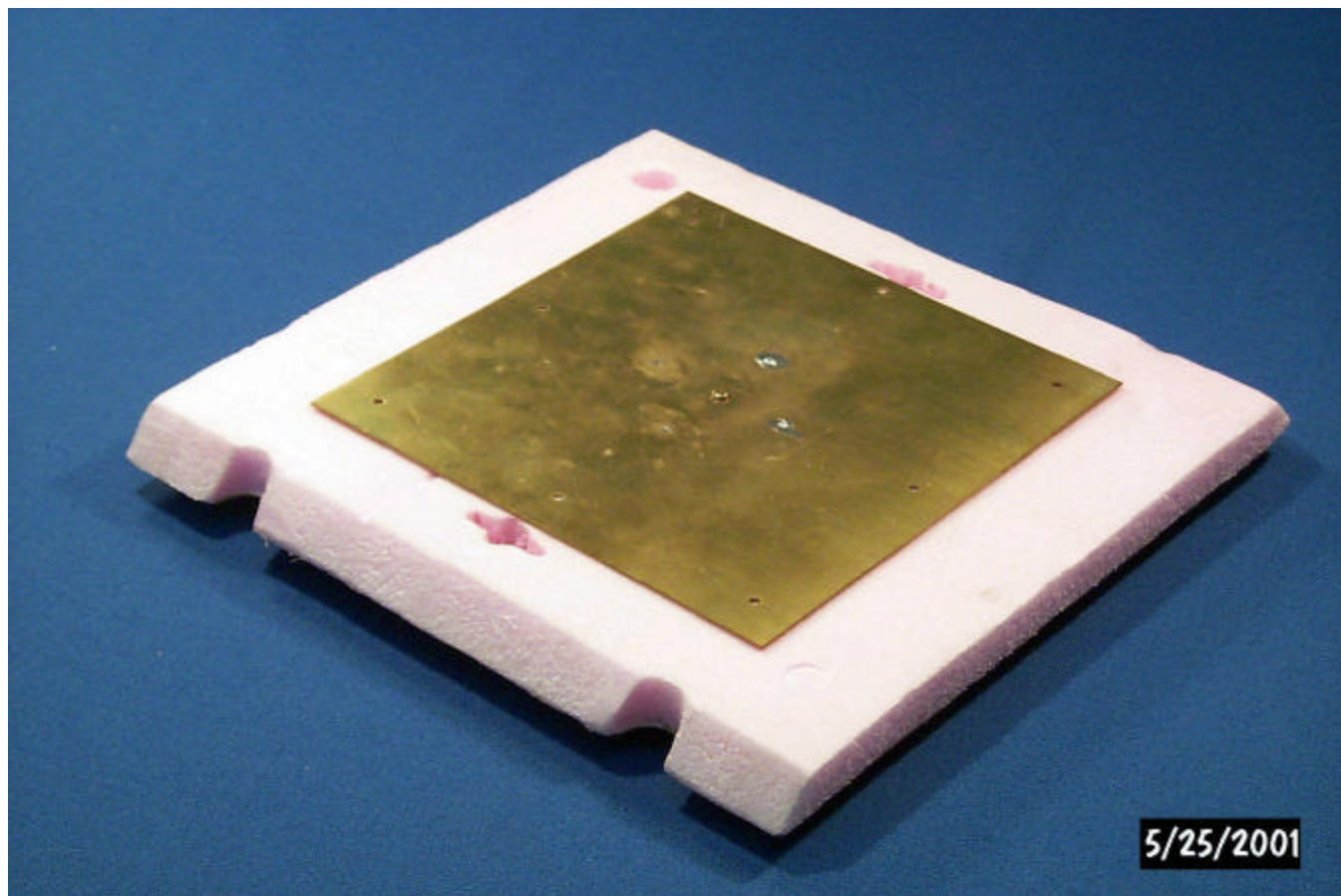
LR-911 Patch Antenna
