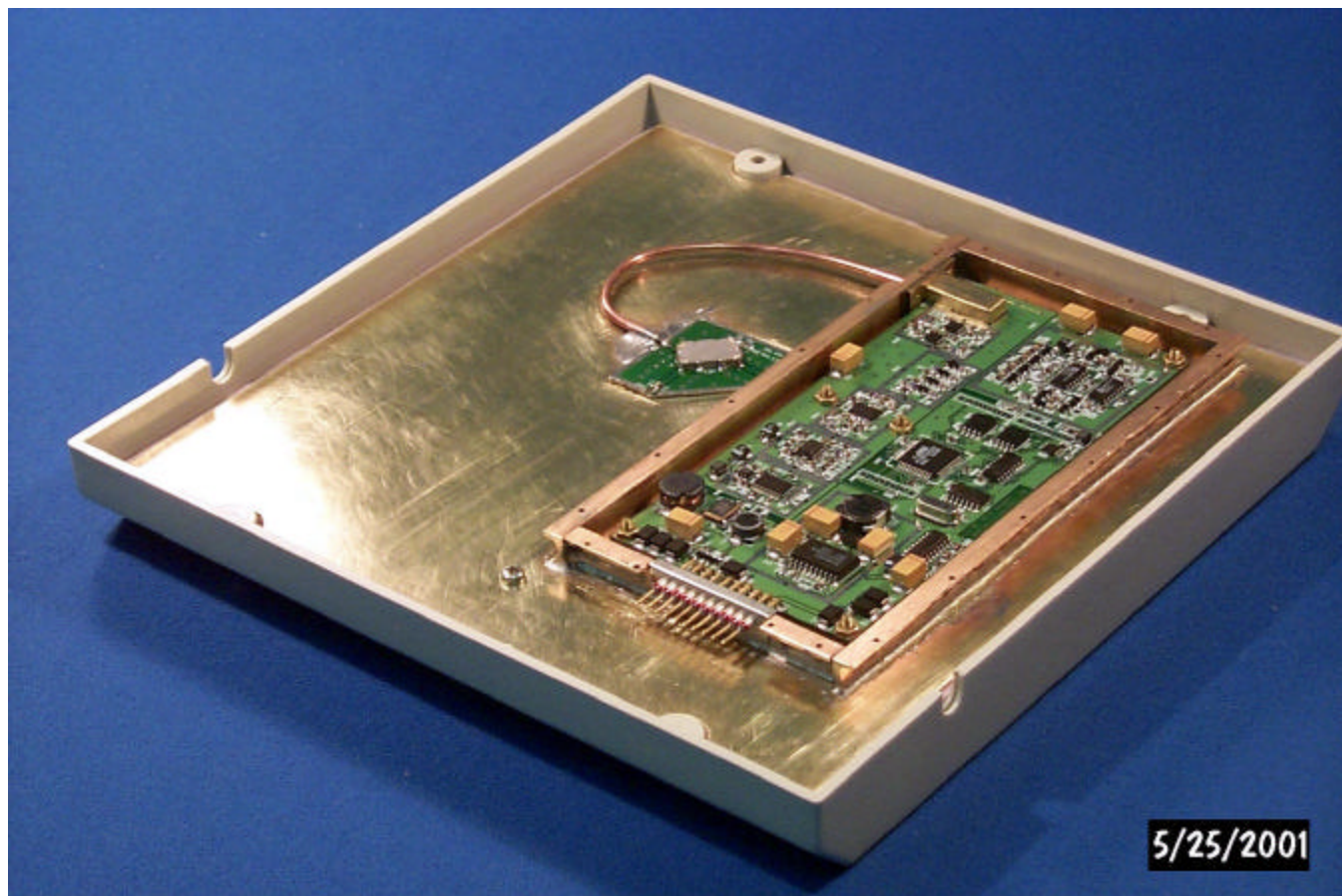
LR-911 without shield
