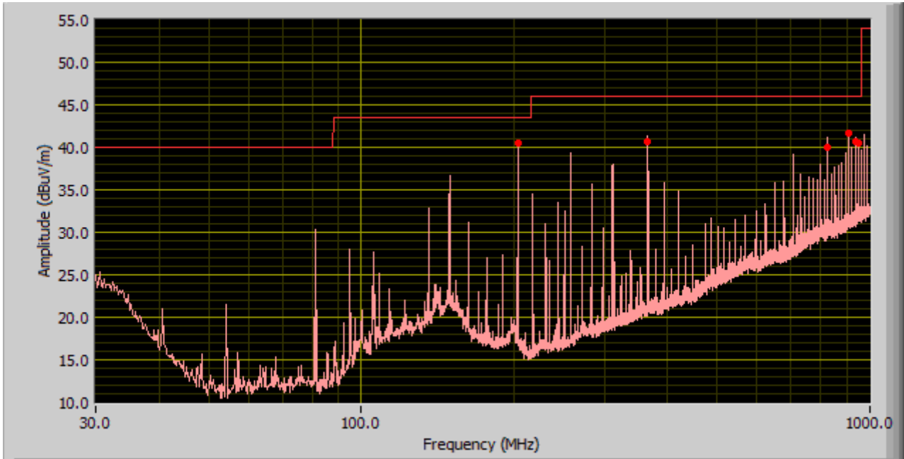
Radiated Emission Test Table 30MHz ~ 1000MHz
