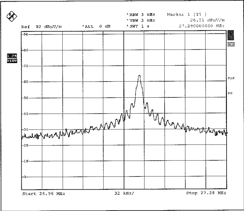
Bandwidth Plot
