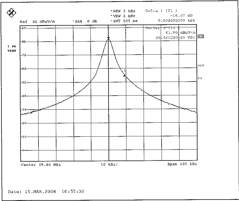
Bandwidth Plot
