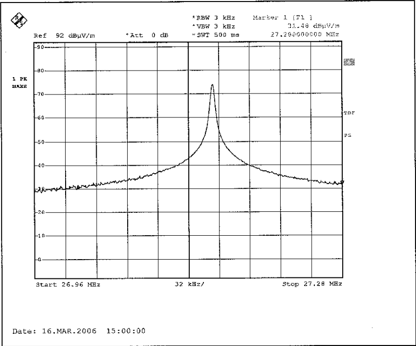
Bandwidth Plot
