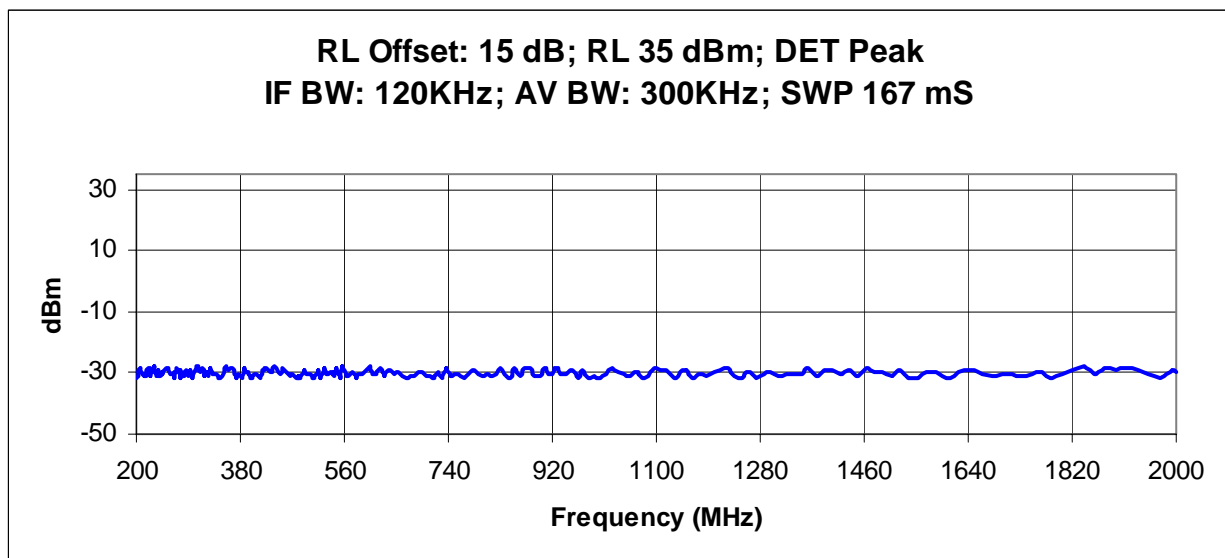
Plot 9: Conducted Spurious Emissions High Ch
