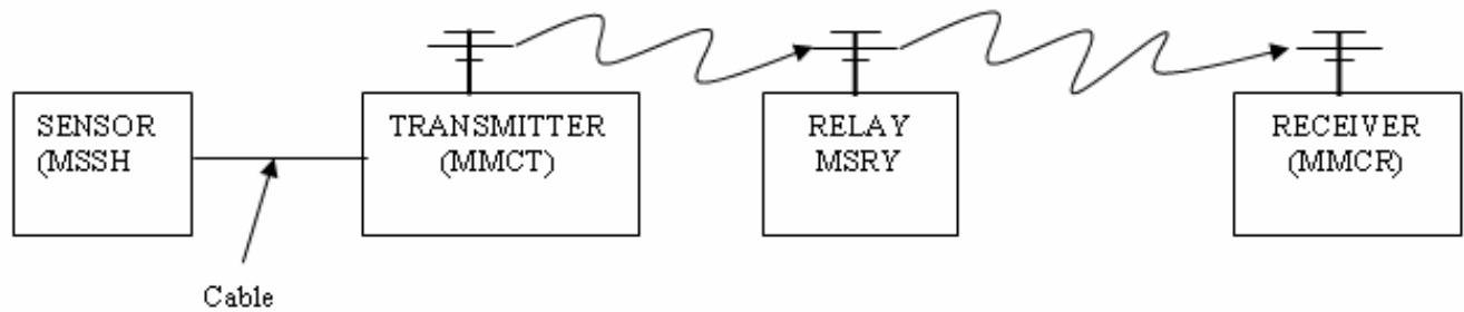
Figure 1. Block Diagram of Test Configuration (Radiated Emissions)
