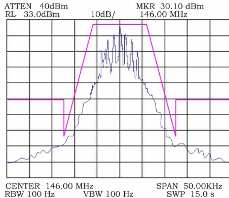
Plot 1. Emission Mask Low Ch
