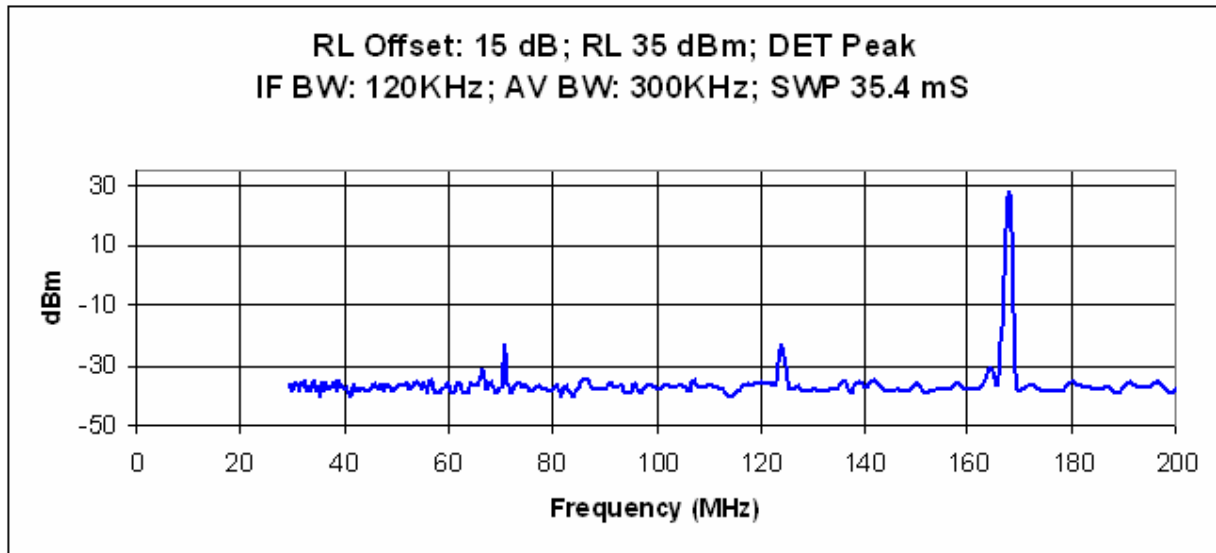
Plot 8. Conducted Spurious Emissions High Ch
