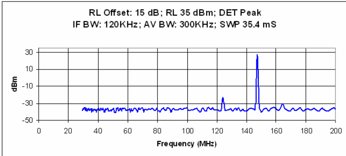
Plot 4. Conducted Spurious Emissions low Ch
