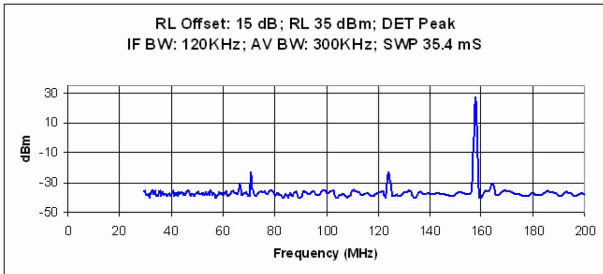
Plot 6: Conducted Spurious Emissions Mid Channel
