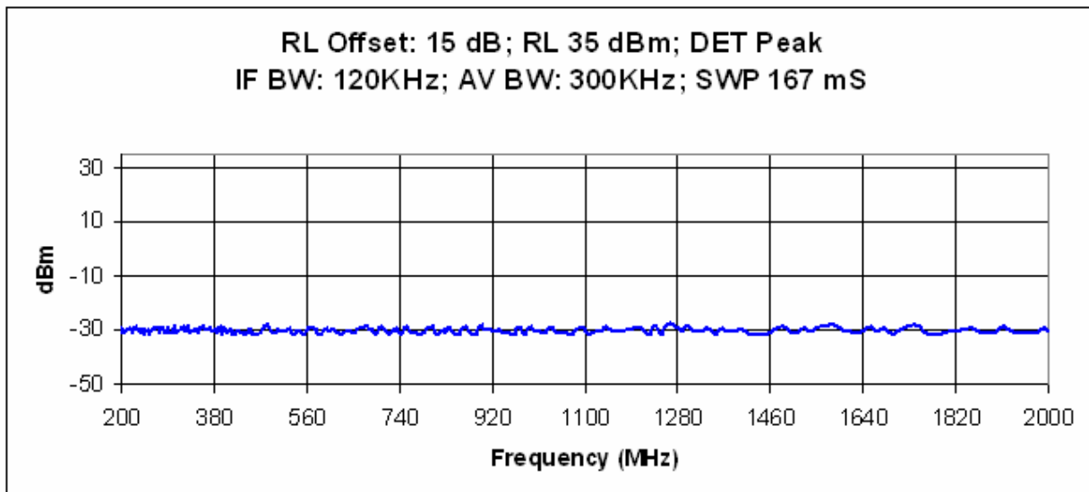
Plot 7: Conducted Spurious Emissions Mid Channel
