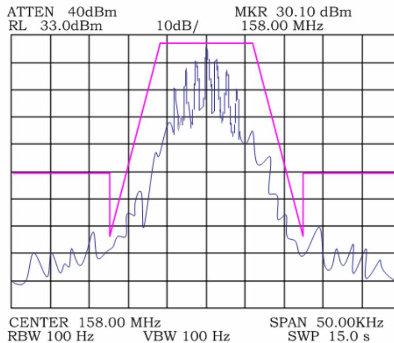
Plot 2. Emission Mask Mid Ch
