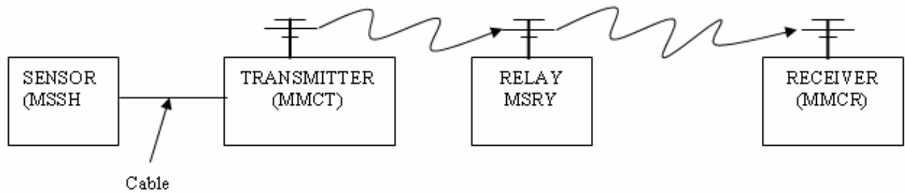
Figure 1. Block Diagram of Test Configuration (Radiated Emissions)
