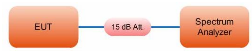
Figure 4. Spurious Emissions at Antenna Terminals Test Setup
