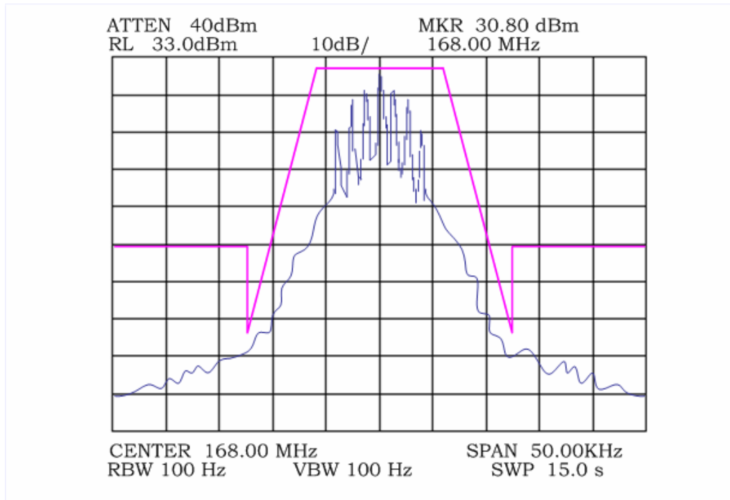
Plot 3. Emission Mask High Ch
