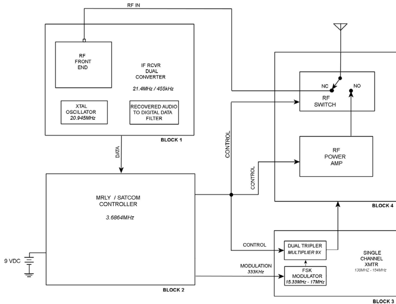
MRLY BLOCK DIAGRAM
