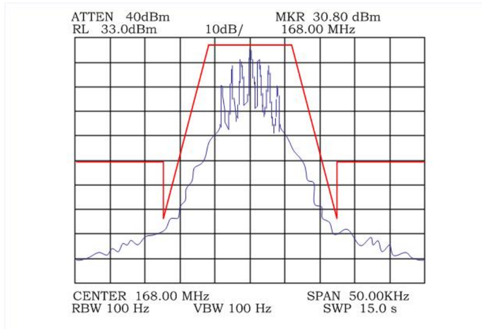
Plot 3. Emission Mask High Ch
