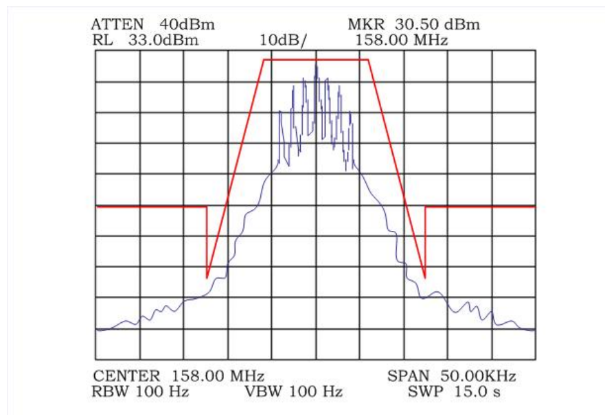
Plot 2. Emission Mask Mid Ch
