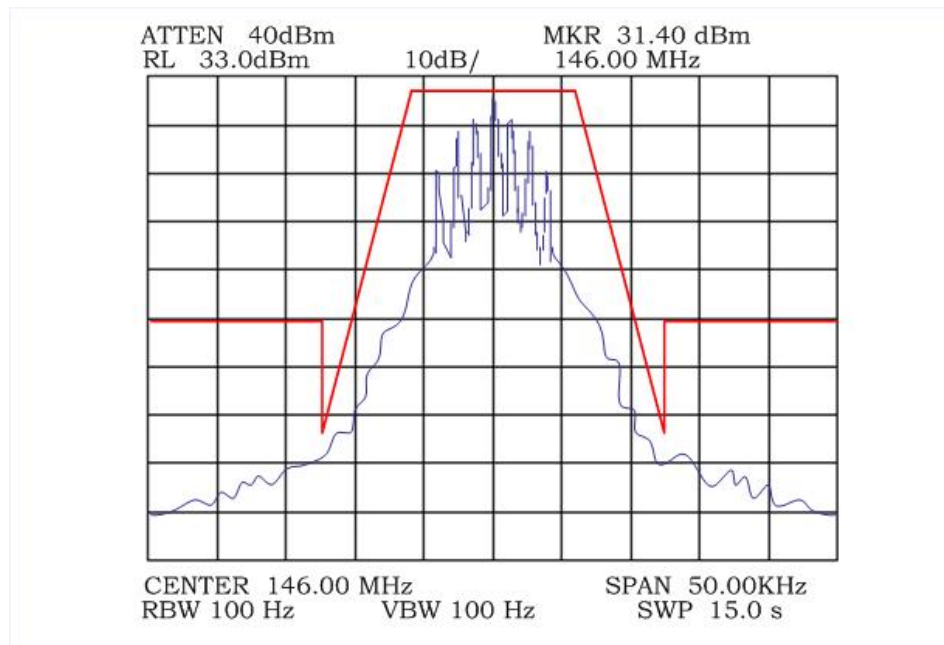
Plot 1. Emission Mask Low Ch
