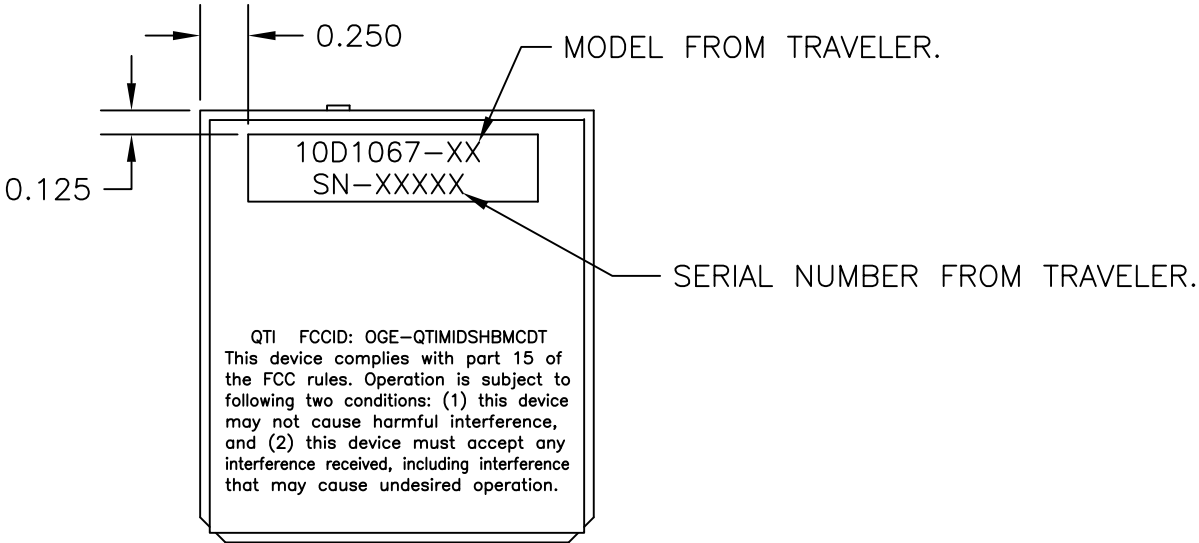
BOTTOM SHIELD OF MCDT HIGH BAND
