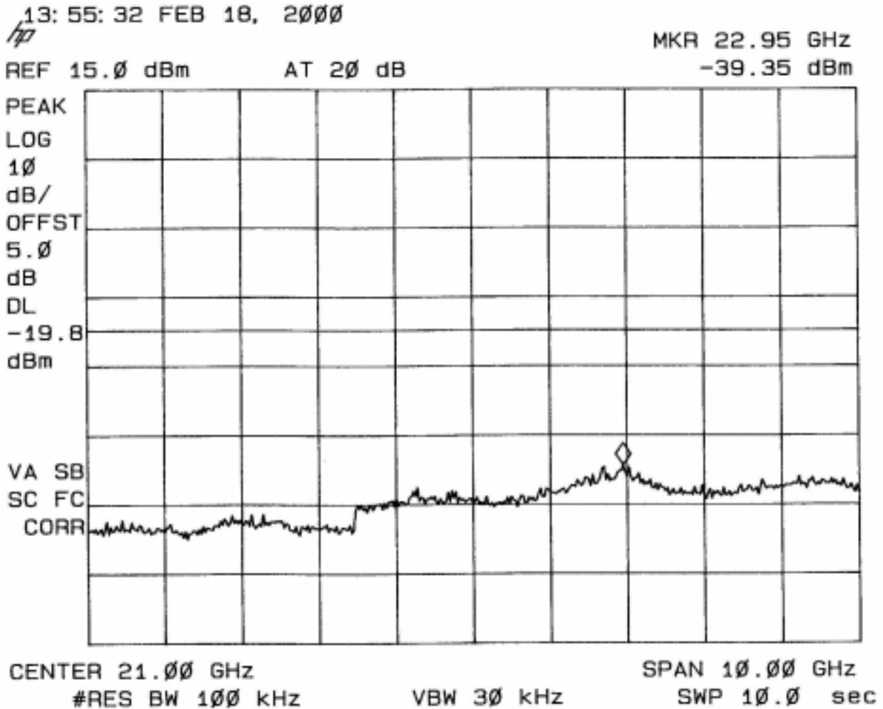
Plot 9.7: Conducted emissions 16.0 – 26.0 GHz
