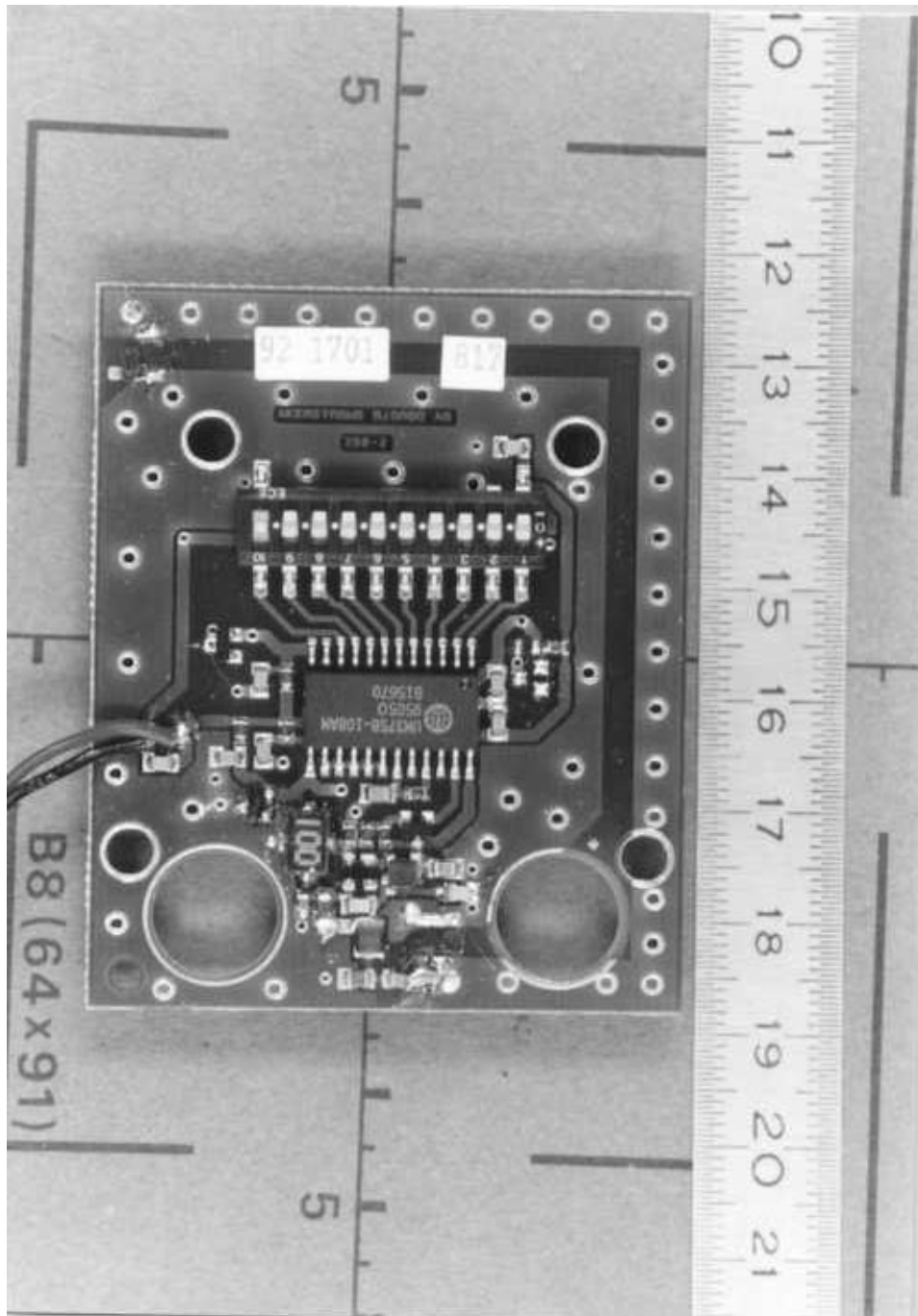
Top view - printed board - Sesam 503
