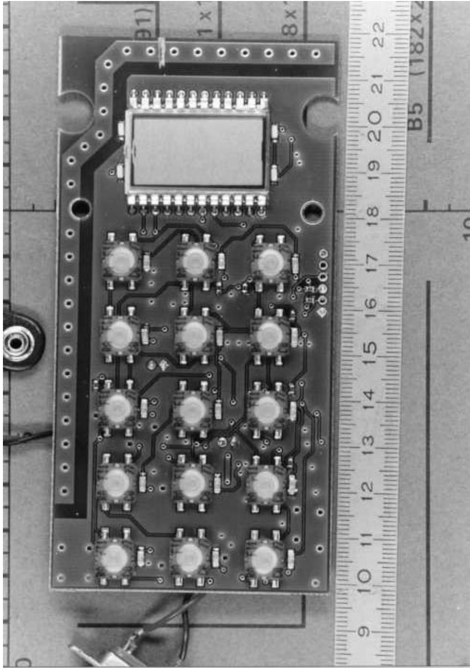
Bottom view - printed board - Sesam 599
