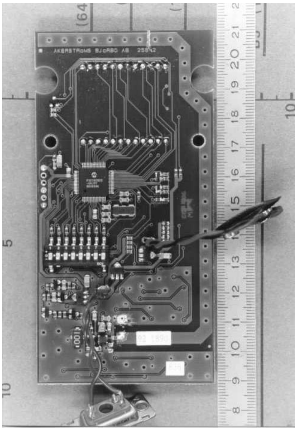
Top view - printed board - Sesam 599
