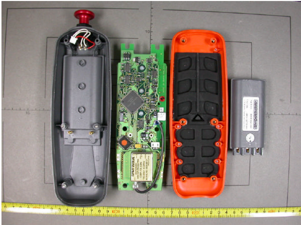
EUT disassembled
