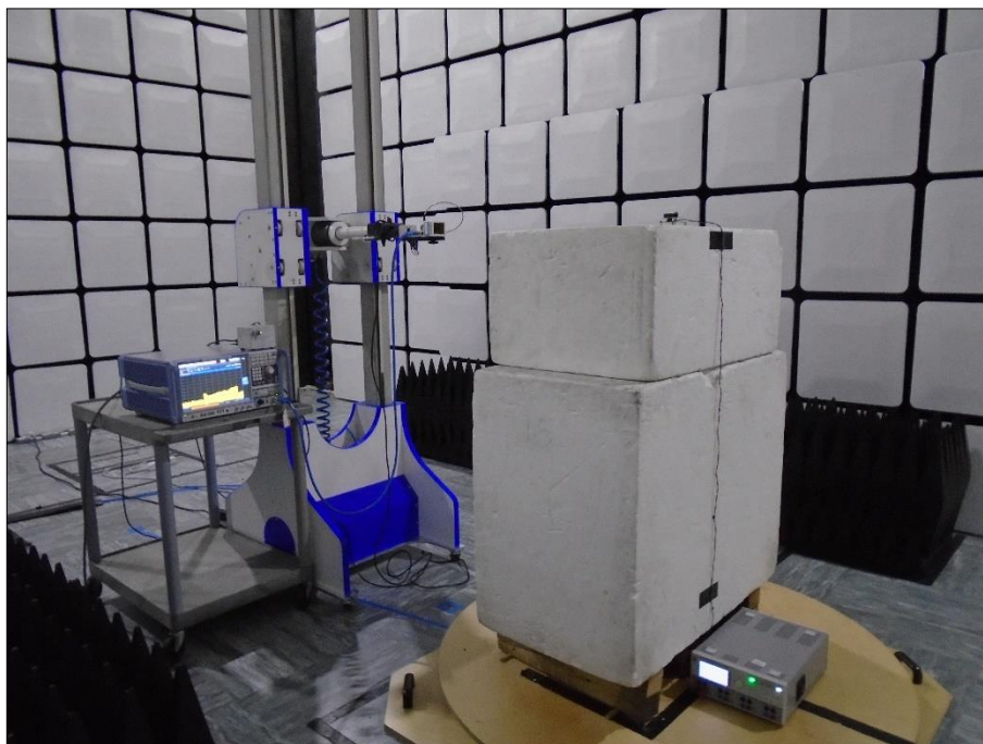
Figure 4 - Test Setup - 18 GHz to 25 GHz
