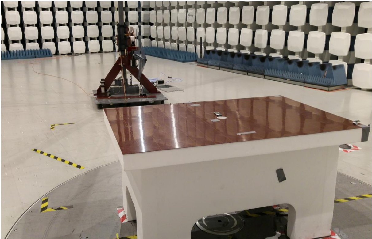
Radiated emission 200 -1000 MHz
