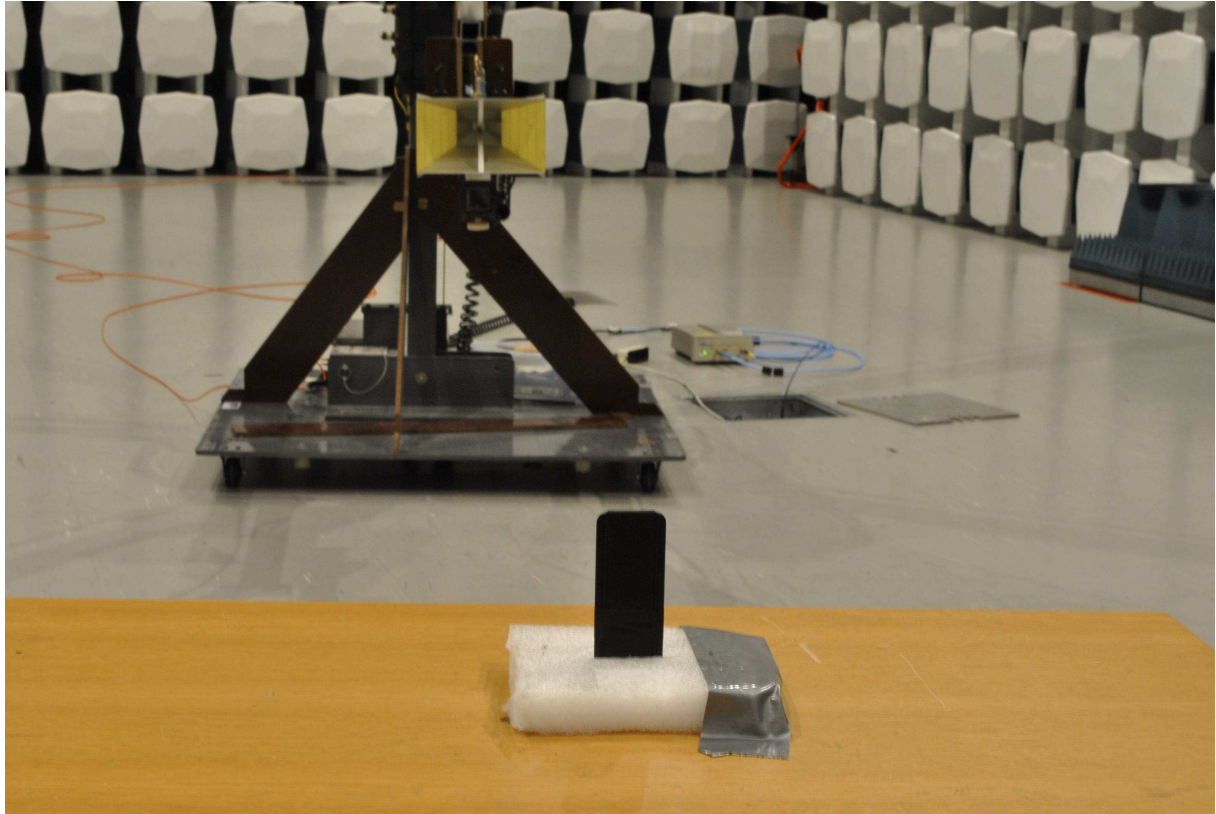
XY plane - Radiated Emissions
