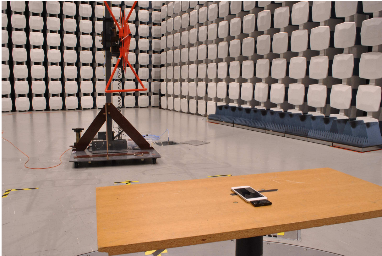
Radiated Emissions
