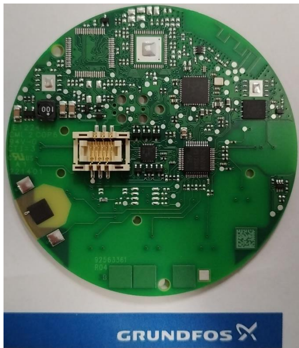
Figure 2 – Bottom side of 92710890 Module
