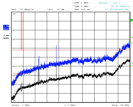
Radiated Emissions 1 - 18 GHz, 2435 MHz, VP
