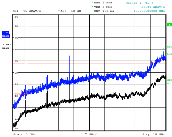
Radiated Emissions 1 - 18 GHz, 2405 MHz, HP
