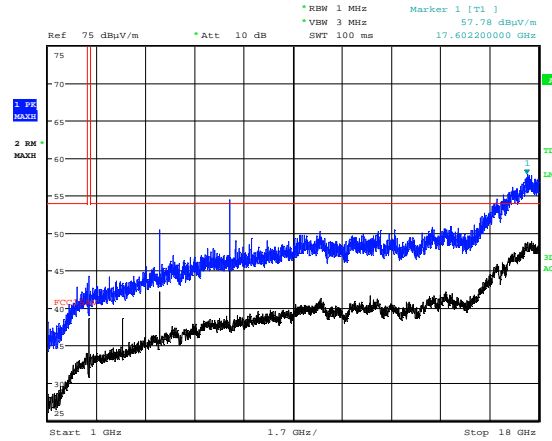
Radiated Emissions 1 - 18 GHz, 2405 MHz, VP
