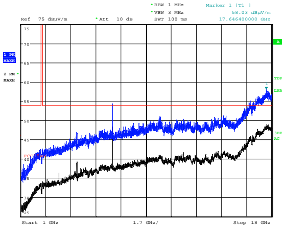
Radiated Emissions 1 - 18 GHz, 2405 MHz, HP
