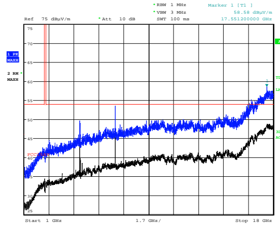
Radiated Emissions 1 - 18 GHz, 2405 MHz, VP
