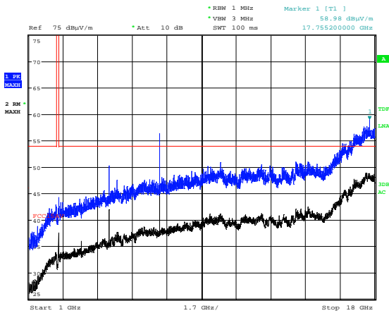
Radiated Emissions 1 - 18 GHz, 2435 MHz, HP
