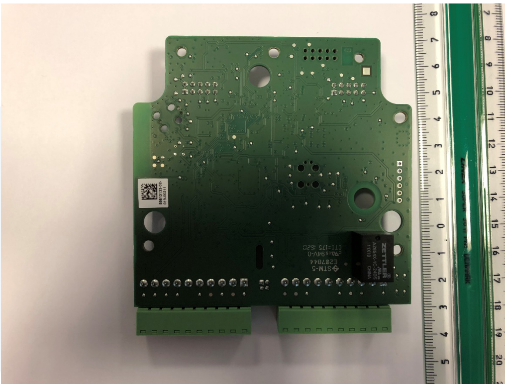
Rear side
