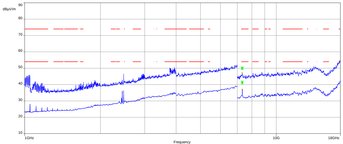
Plot 2: 1 GHz to 18 GHz, TX mode, 2442 MHz, vertical & horizontal polarization, 1 Msps
