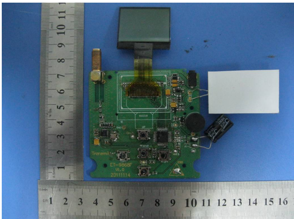
Uncovered-Main PCB – Front View
