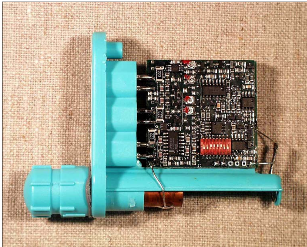
Figure 5: PCB - Rear View
