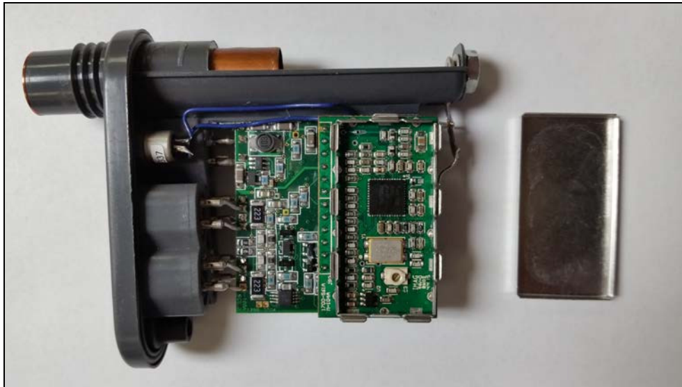
Figure 3: PCB with Shield Removed
