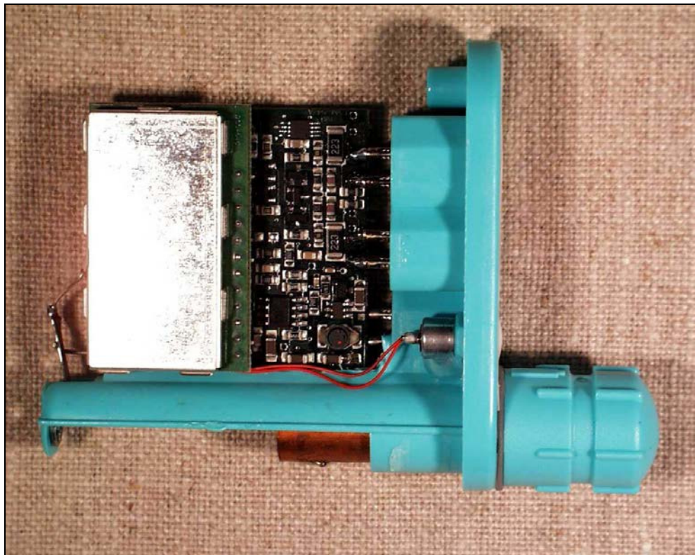
Figure 2: PCB and RF Boards Assembled - Top View
