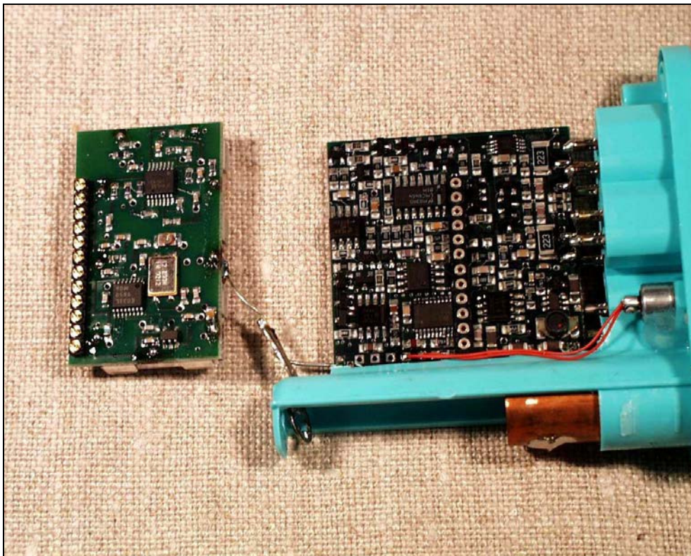
Figure 4: PCB and RF Board Assembly with RF Board Removed
