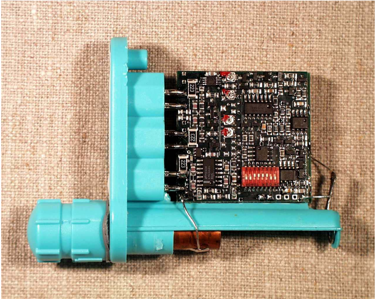
Figure 4: PCB rear view
