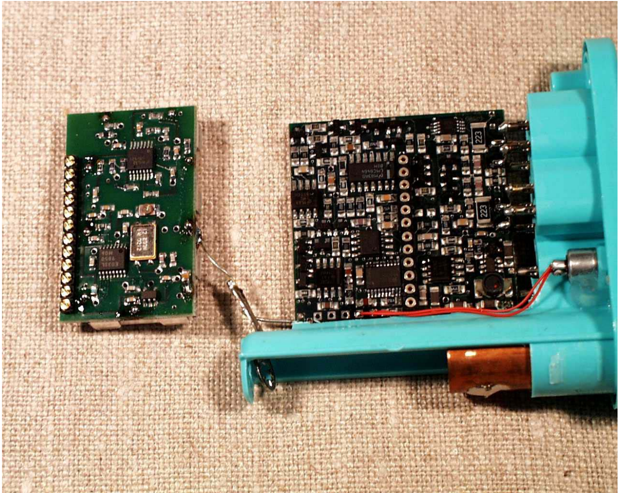
Figure 3: PCB and RF board assembly with RF board removed
