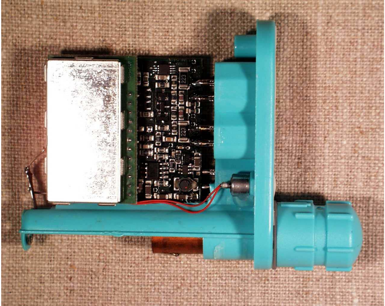
Figure 2: PCB and RF boards assembled, top view
