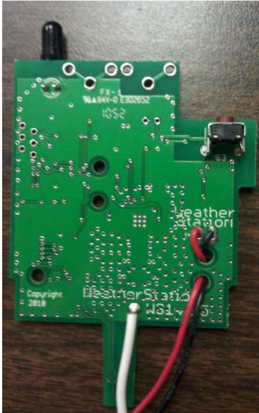
7.5 PCB Foil View
