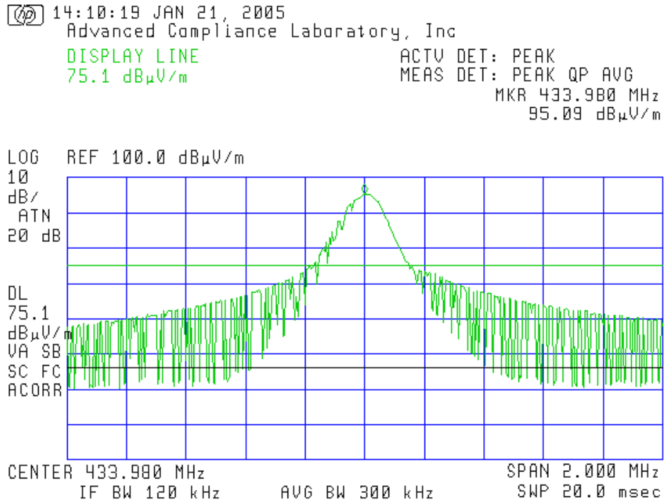
Figure 5.2 Occupied Bandwidth
