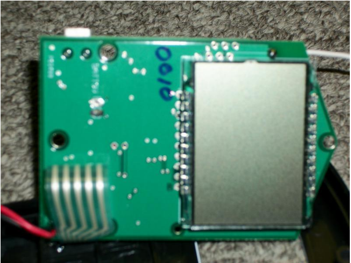
7.5 PCB Foil View
